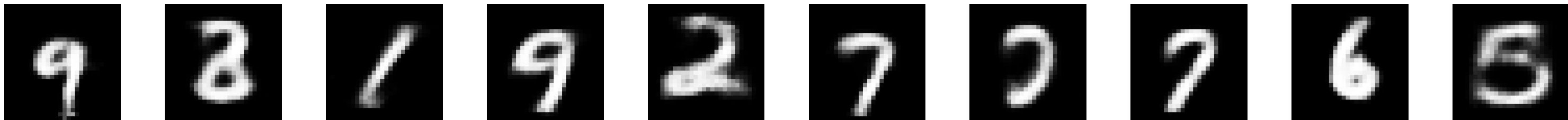
CAE Recon.
